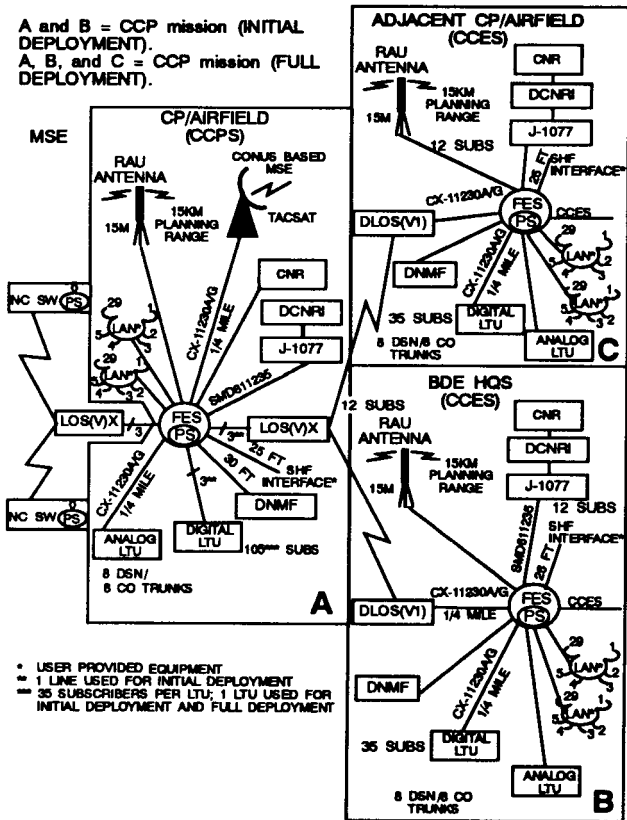
Figure 3-13. CCP conventional mission in its entirety.
