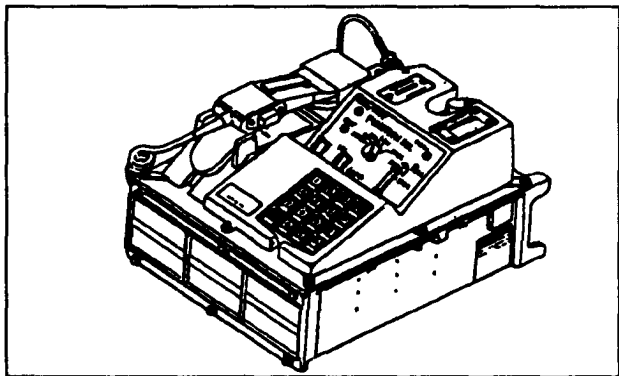
Figure 3-30. DSVT, TSEC/KY-90.
