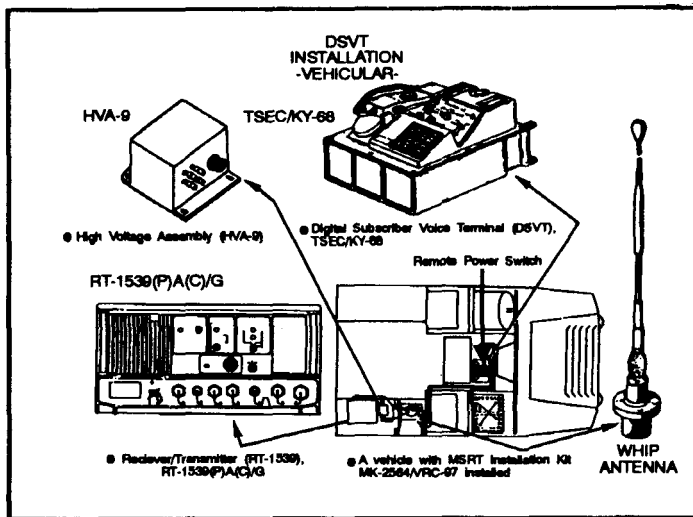
Figure 3-31. Vehicle mounted (MK-2564/AN/VRC-97) MSRT.
