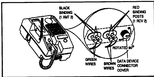
Figure 3-29. DNVT, TA-1035/U and field wire connections.
