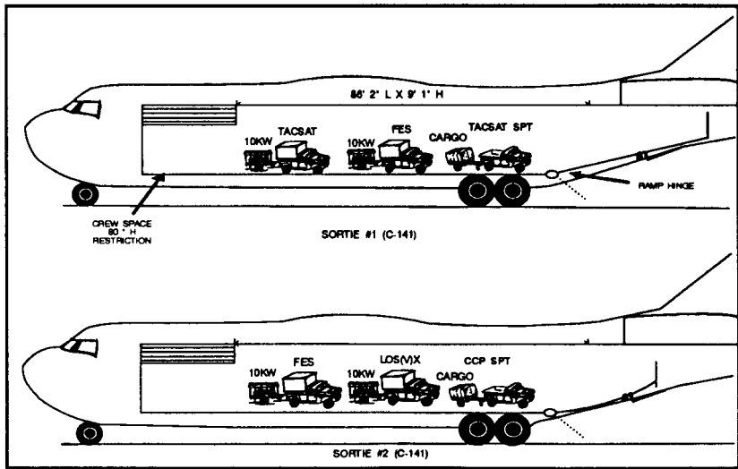
Figure 3-14. CCP initial deployment.
