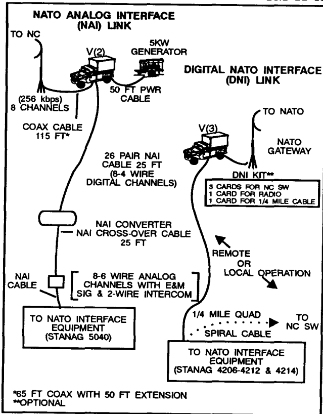
Figure 3-8. Typical LOS(V)2 NATO analog interface link and LOS(V)3 digital NATO interface link.
