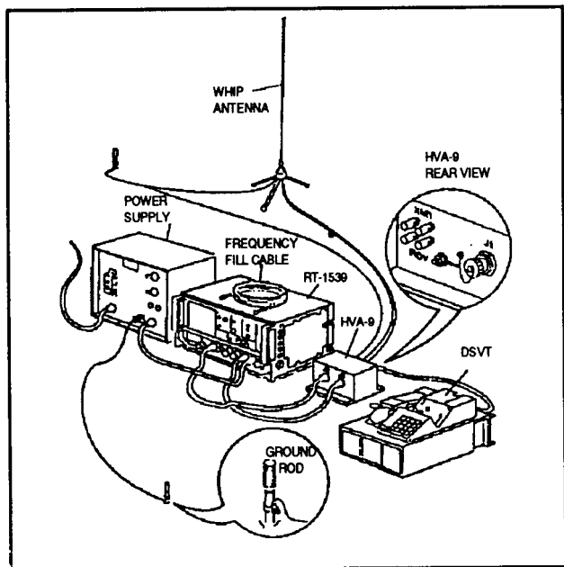
Figure 3-32. Stand-alone kit (MK-2565/AN/VRC-97) with MSRT.
