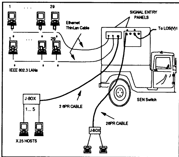
Figure 3-23. TPN host connectivity at a SEN.
