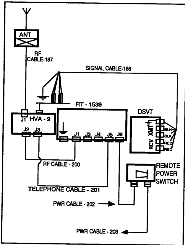
Figure 3-33. MSRT wiring diagram.
