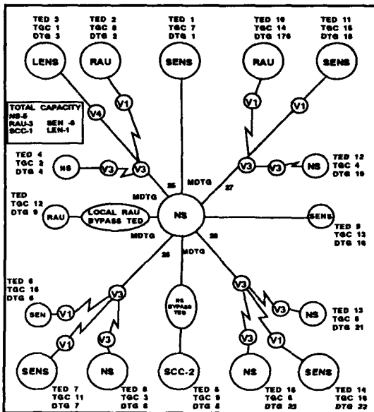
Figure 3-20. NC switch DTG/TGC standard database.
