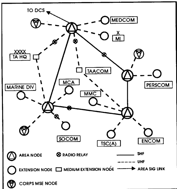
Figure 3-25. TRI-TAC area communications system.
