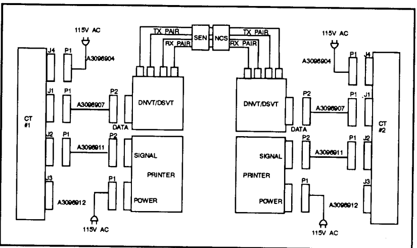
Figure 3-40. CT communications via MSE.
