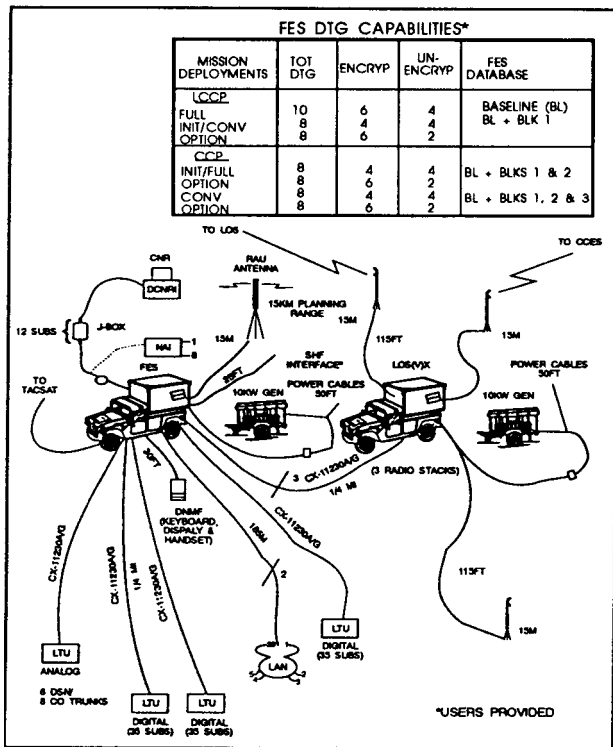
Figure 3-15. Typical CCPS deployment.
