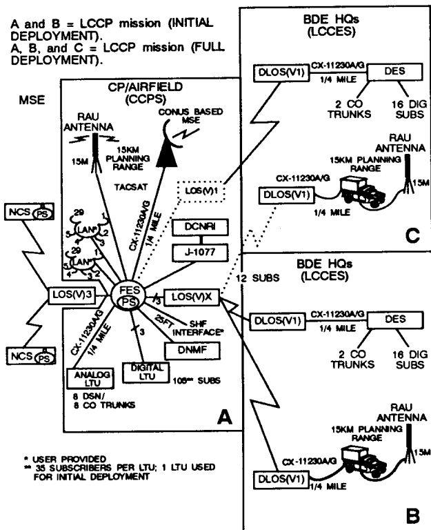
Figure 3-18. LCCP conventional mission in its entirety.
