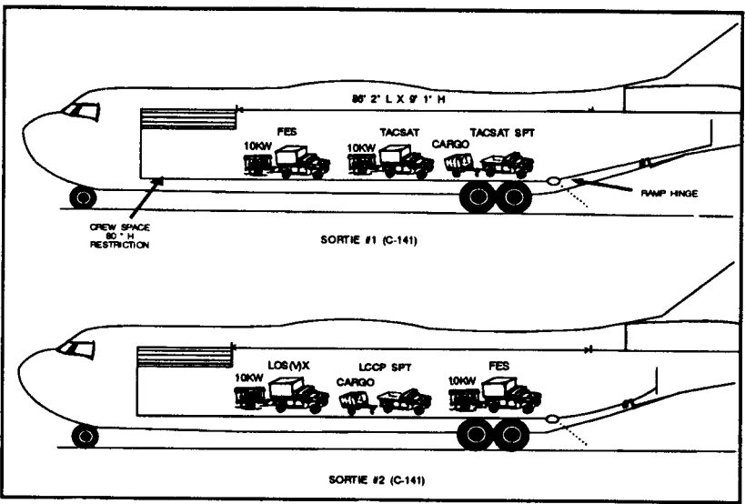
Figure 3-19. LCCP initial deployment.
