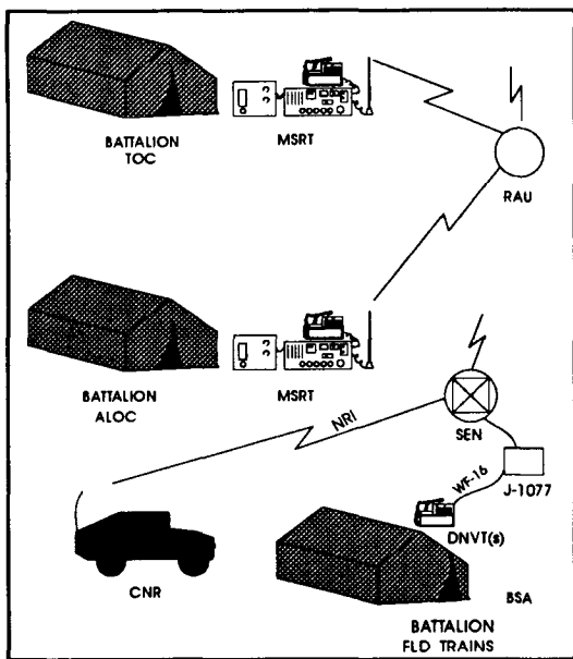
Figure 2-5. Battalion ACUS access.
