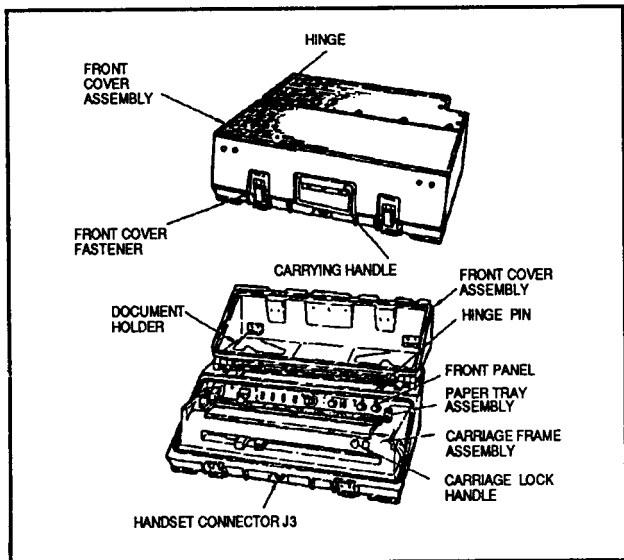
Figure 3-35. LDF, AN/UXC-7/7A.
