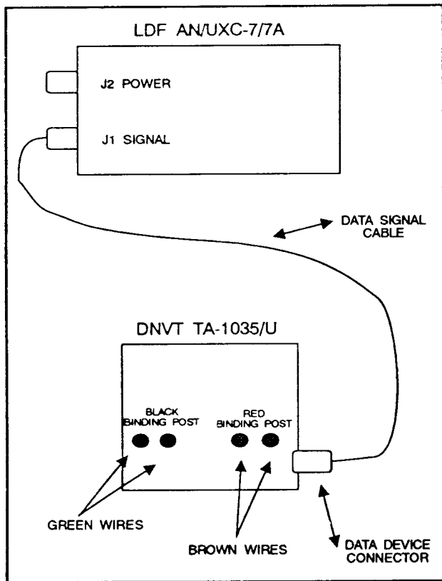
Figure 3-38. MSE telephone interface to LDF.
