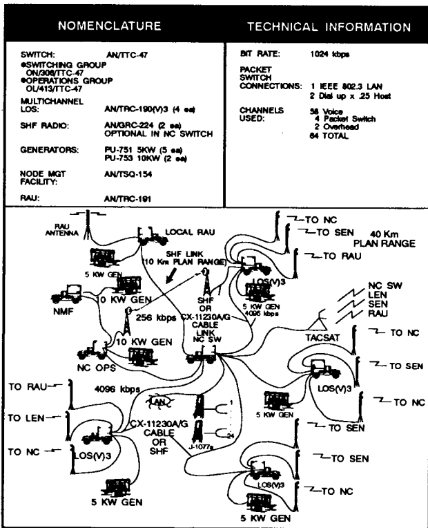
Figure 3-3. Typical NC configuration.
