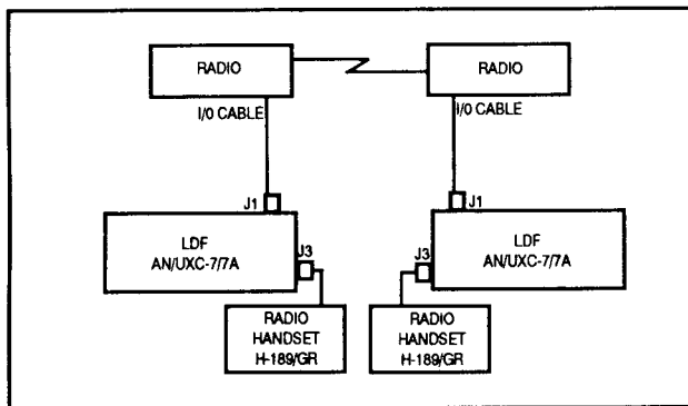
Figure 3-37. Radio interface to LDF.
