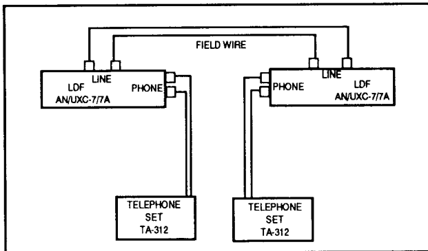
Figure 3-36. Phone line interface to LDF.
