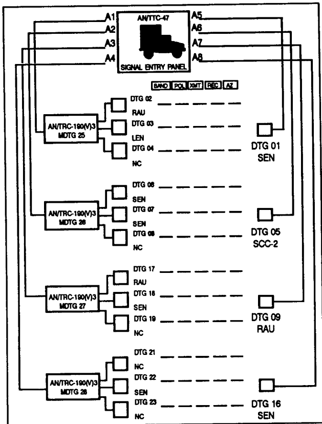
Figure 3-24. NC switch trunk status diagram.
